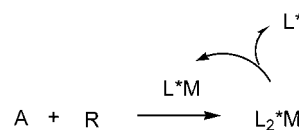
Figure 5. Schematic representation of the present self-replication in asymmetric aminohydroxylation.
