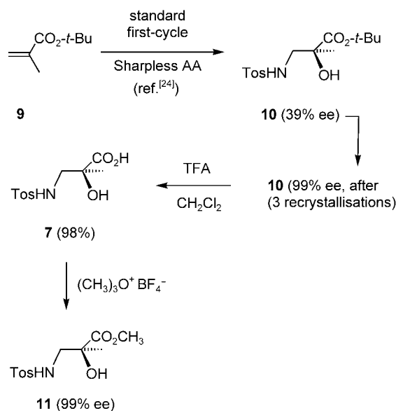
Scheme 1. Synthesis of ligand 7 .
