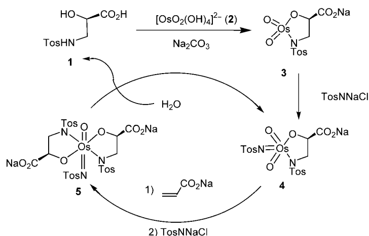
Figure 2. Catalytic cycle for self-replication in asymmetric aminohydroxylation.
