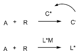
Figure 1. Schematic representation of chiral autocatalysis ( top ) and chiral self-replication ( bottom ).
