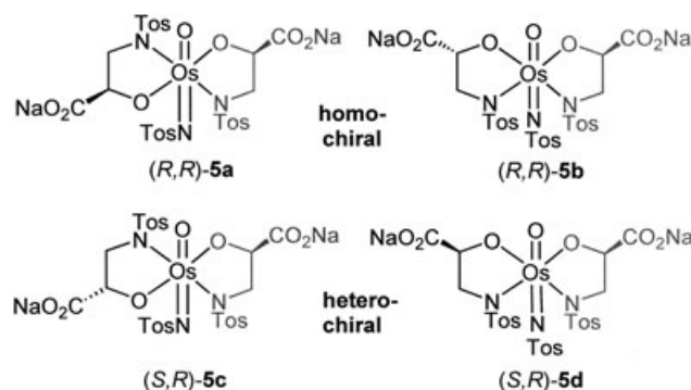
Figure 4. Intermediate bis(azaglycolate) osmium esters.
