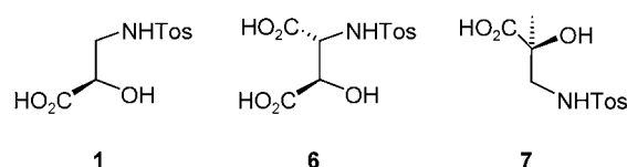
Figure 3. Chiral ligands for self-replication via second-cycle AA reaction.
